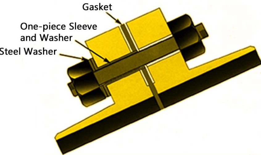
One-piece sleeve & washer configuration
